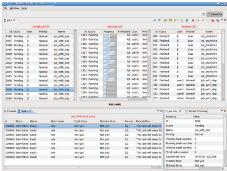
Figure 3: ProActive Scheduler.
